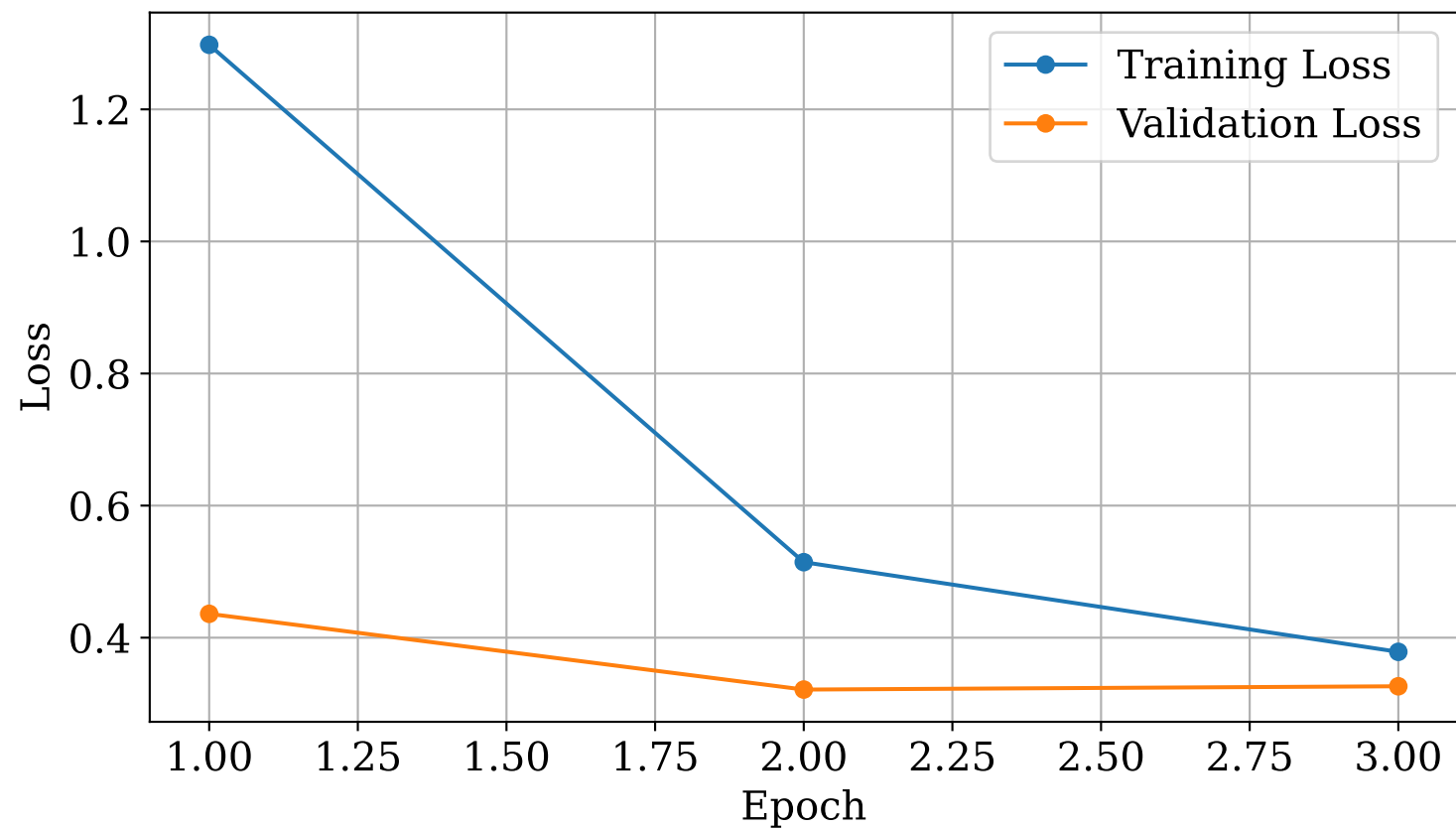
Baseline MobileNetV2 - Loss
